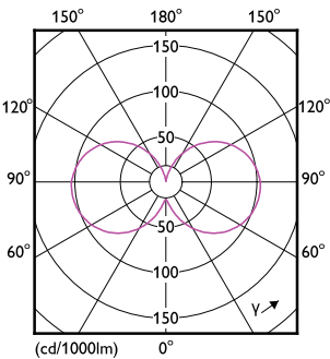
Light Distribution Diagram - CorePro LED PLC 360D 9.5W 3CCT 4P G24q-3
