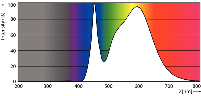
Spectral Power Distribution Colour - CorePro LED PLC 360D 9.5W 3CCT 4P G24q-3
