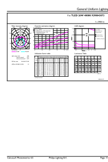
General uniform lighting - MAS LEDtube Mains/EL 1200mm 26W 840 T5
