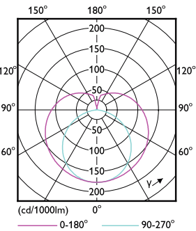
Light Distribution Diagram - MAS LEDtube Mains/EL 1200mm 26W 840 T5
