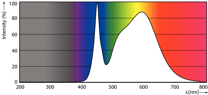
Spectral Power Distribution Colour - MAS LEDtube Mains/EL 1200mm 26W 840 T5
