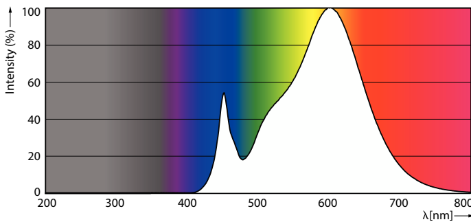
Spectral Power Distribution Colour - CorePro LED PLL HF/Mains 24W 830 4P
