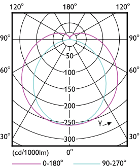
Light Distribution Diagram - MAS LEDtube Mains/EL 600mm 7.6W 840 T8
