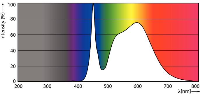
Spectral Power Distribution Colour - MAS LEDtube Mains/EL 600mm 7.6W 840 T8
