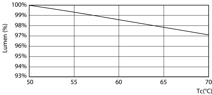
Lumen Maintenance Diagram - MAS LEDtube Mains/EL 600mm 7.6W 840 T8
