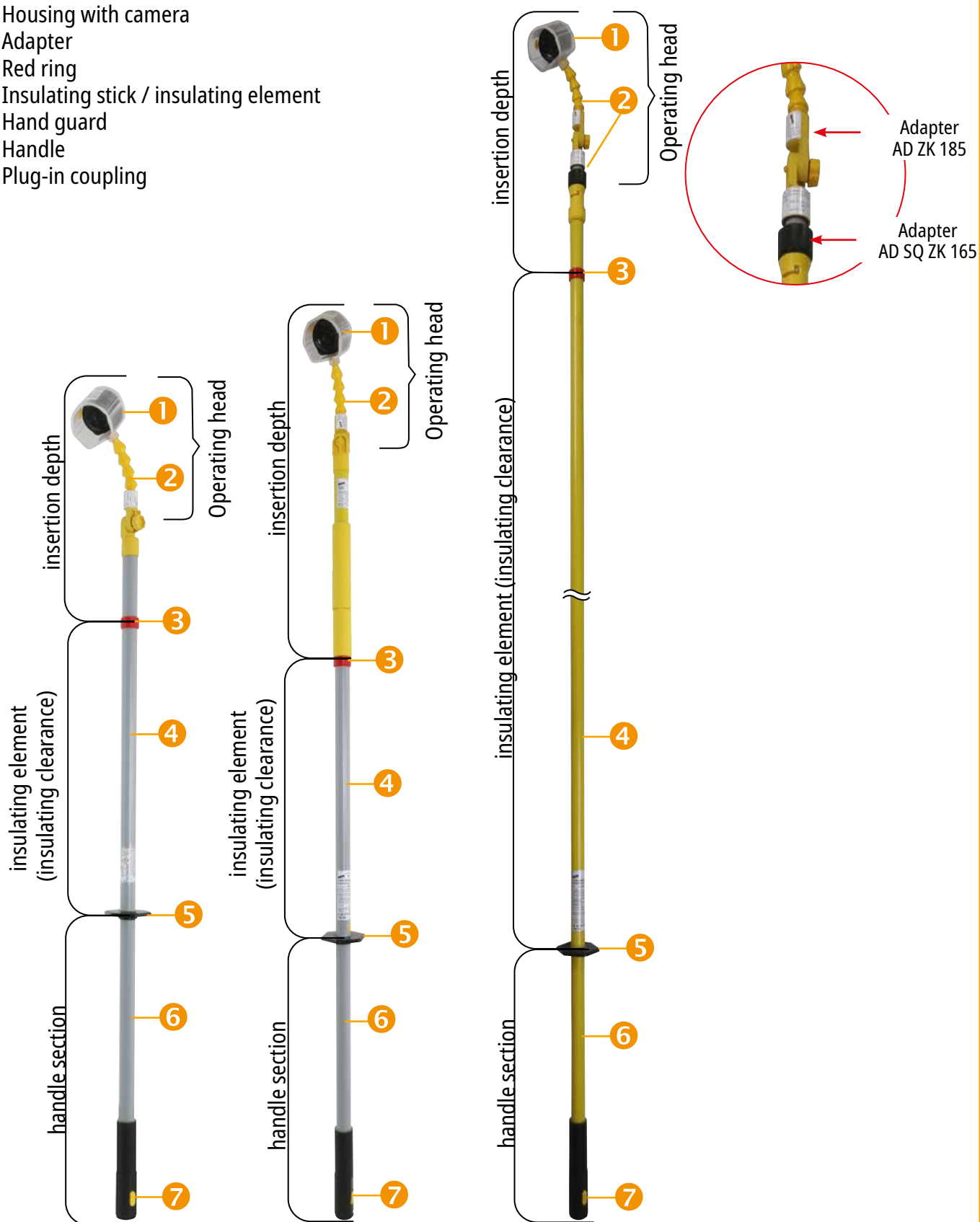
Fig. 10 Insulating stick with operating head
