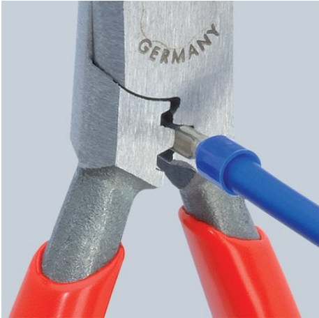
Crimping 0.5 to 2.5 mm²
